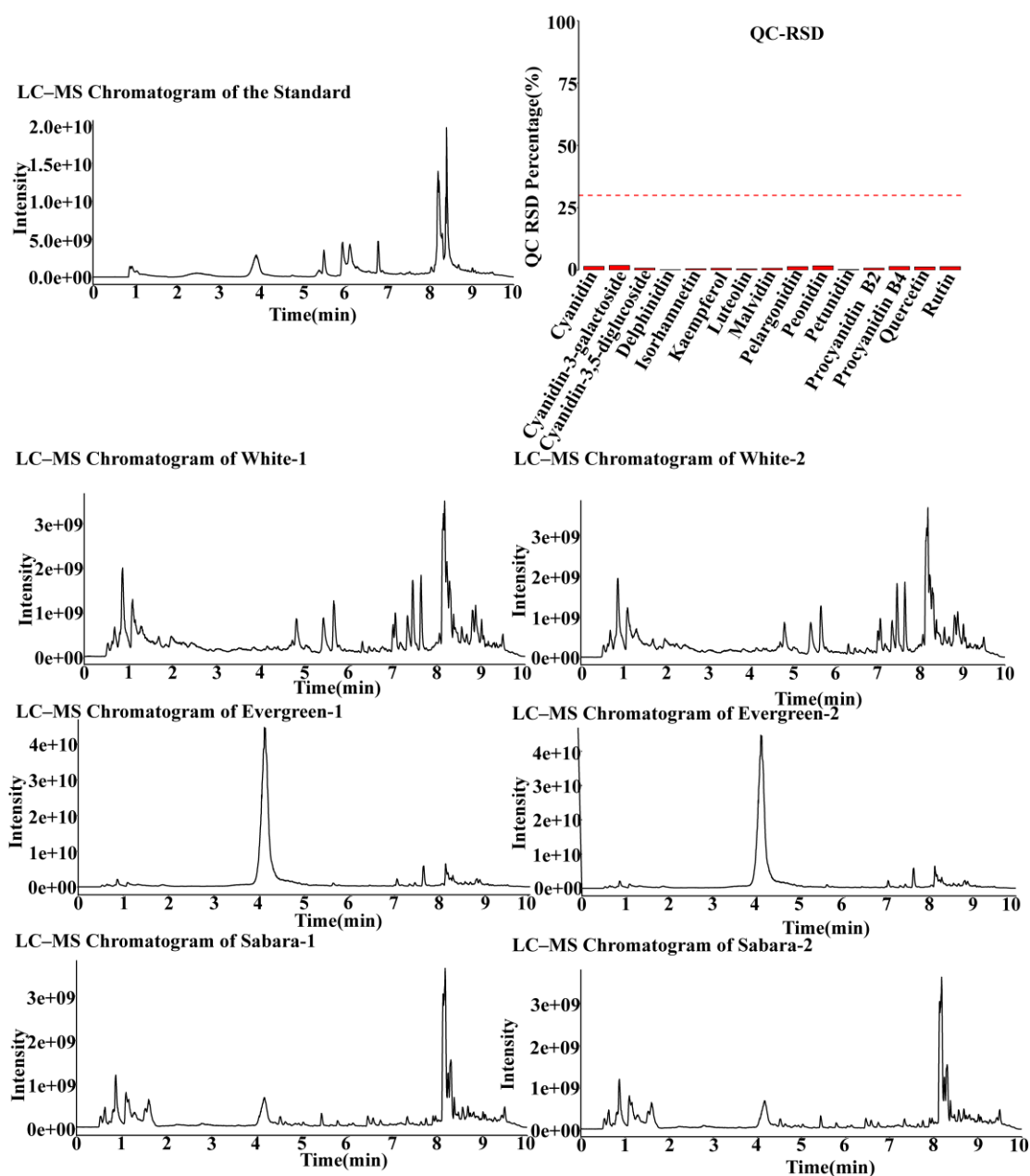
Supplementary Figure S1 Metabolite chromatograms and QC-RSDs.
