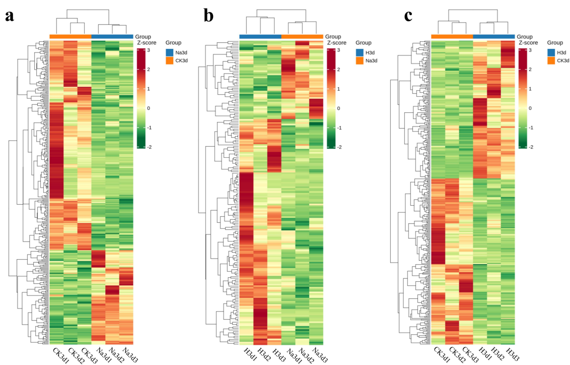
Fig S3. Quality assessment of metabolomic data and variance in DAM accumulation under salt stress and H 2 exposure. (a–c) Hierarchical clustering heatmaps of DAMs across treatments.
