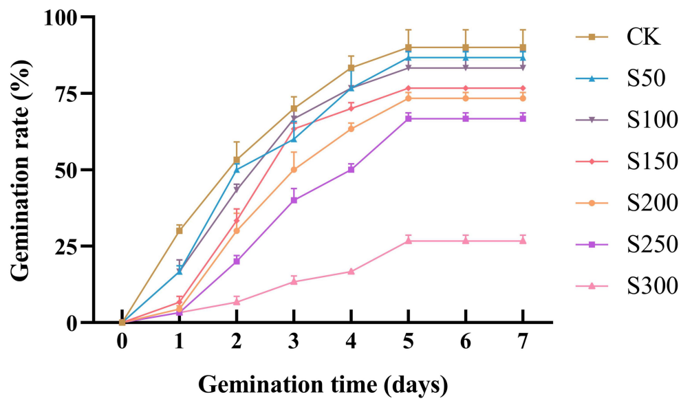
Fig S1 Germination rates of peach seeds at different NaCl concentrations. CK, S50, S100, S150, S200, S250, and S300 represent 0 (distilled water control) and NaCl treatments ranging from 50–300 mmol/L, respectively.
