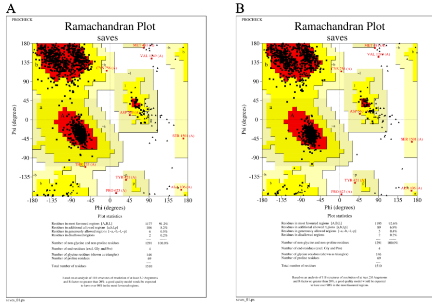
Figure S2: Ramachandran plot of protein structure. A belongs to LrFd-GOGAT; B belongs to LbFd-GOGAT.
