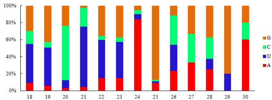
Figure S2. Proportion of the first nucleotide bias within novel miRNAs of the same length in the three libraries of peach sRNAs.
