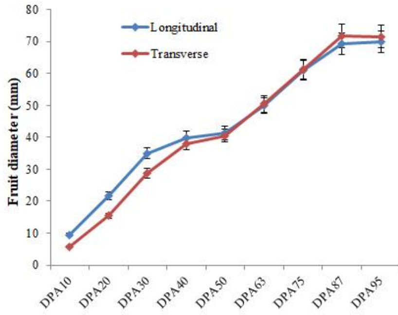
Figure S1. Changes in the longitudinal and transverse diameters of 'Baifeng' peach during different developmental stages.
