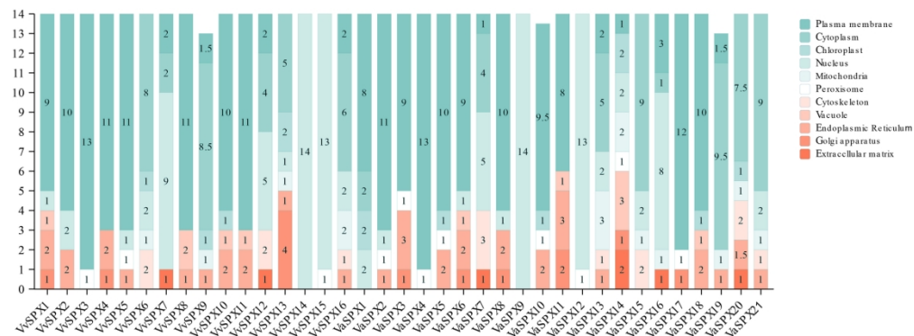
Subcellular localization of SPX protein in Vitis vinifera and Vitis amurensis . The numbers in the bar chart represent the number of subcellular localization.
