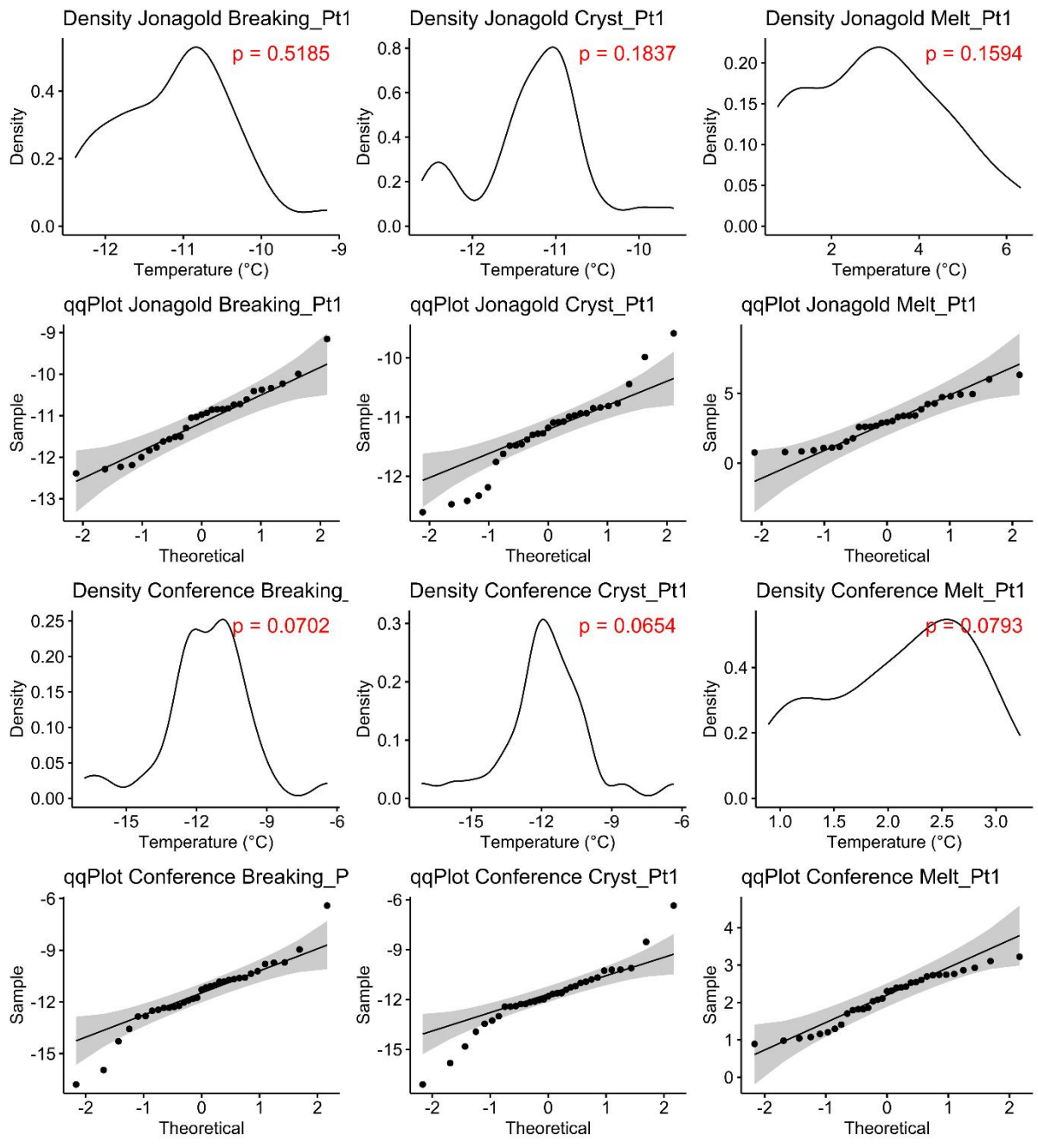
Figure S2 Density and qq plots for the recorded temperature data (i.e. breaking, crystallization, and melting points) of the first freezing-thawing cycle. “p” shows the Shapiro-Wilk p -value for each measured data point.
