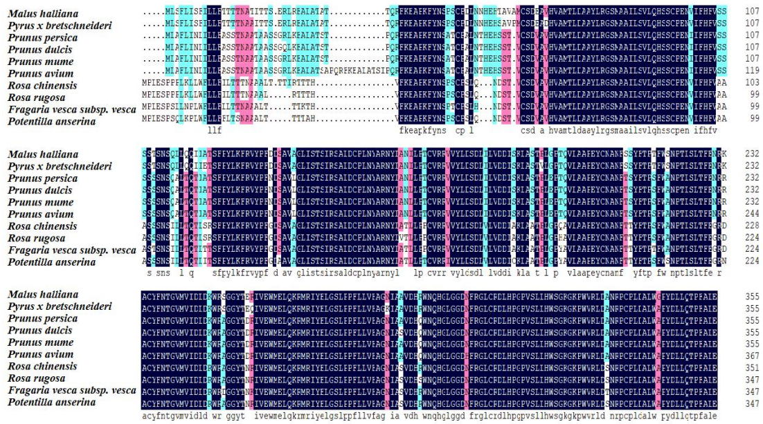
Figure S4 Sequence comparison between the MhGATL1 and other species
