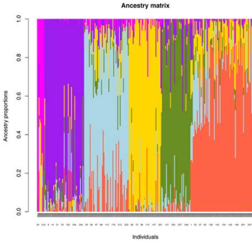
Supplementary Figure S5. Population structure plot. Calculated for 2,293 SNPs and 264 individuals.
