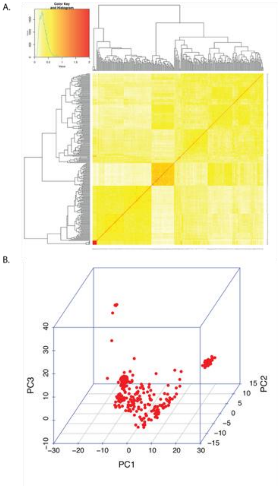
Supplementary Figure S6. Kinship relationships and 3-D Principal Component Plot. A. Heatmap with kinship values (0-2) with dendrogram for 264 individuals B. Displays the distinct groupings for the sampled families.
