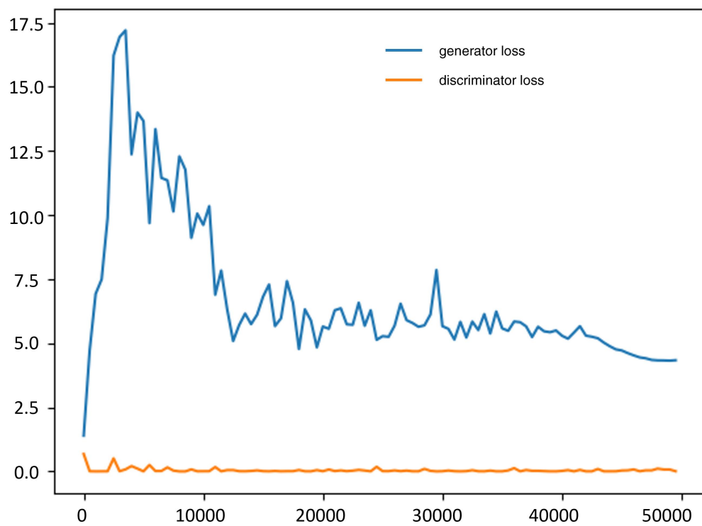
Figure S1: Loss functions of cGAN generator (blue) and discriminator (green) networks during training.
