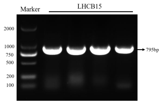
Supplemental Figure S4. Amplified fragment size of MhLHCb15 gene in Malus halliana .
