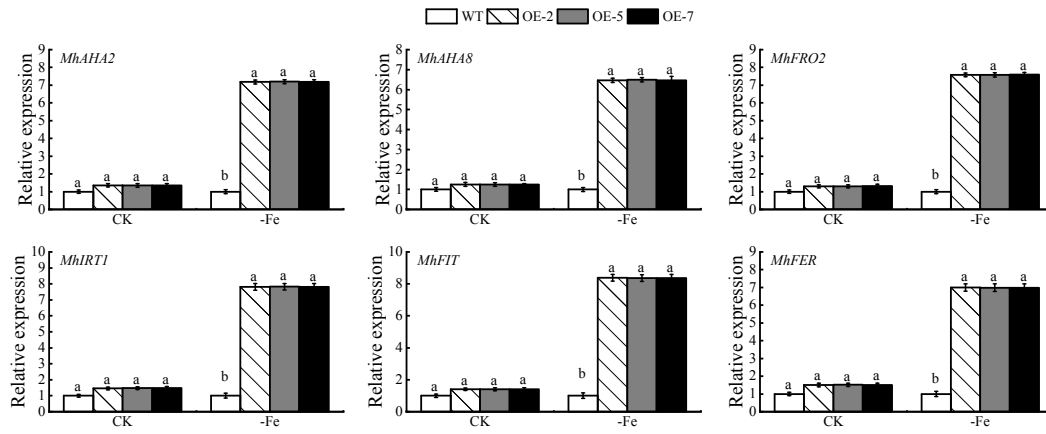
Supplemental Figure S10. Expression of genes related to Fe absorption in overexpressed MhLHCB15 and wild type (WT) A. thaliana grown for 20 days under Fe-sufficient (CK) or Fe-deficient (-Fe) conditions.
