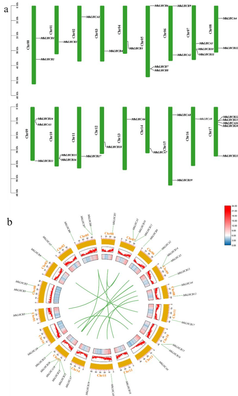
Supplemental Figure S1. Chromosome locations and the collinearity analysis for MhLHC genes family. a Chromosome locations b collinearity analysis of MhLHC genes family. Thick green lines indicate duplicated MhLHC gene pairs. Gene names are shown in black font. Chromosome number is indicated at the bottom of each chromosome. Scale bars marked on each chromosome indicates chromosome length (Mb).
