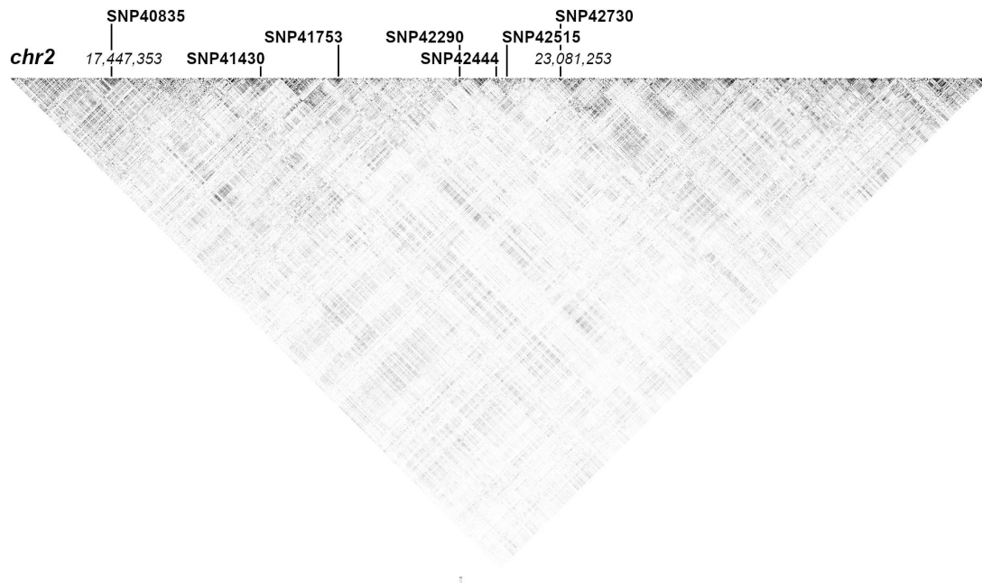
Supplementary Figure 7. Linkage disequilibrium pattern around qMcr2.1 on chr 2.
