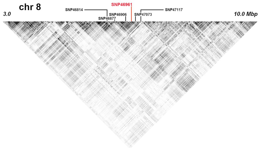
Supplementary Figure 6. Linkage disequilibrium pattern around qMcr8.1 on chr 8.
