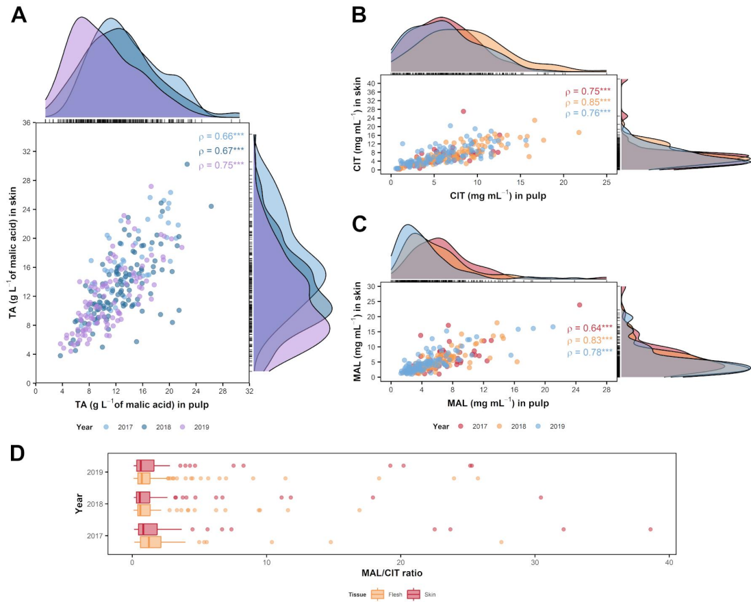
Supplementary Figure 3. Phenotypic variation and Spearman's correlation coefficient between pulp and skin contents in the apricot accession panel along three harvesting seasons for A) titratable acidity (TA, in \text{g L}^{-1} of malic acid), B) citrate (CIT, in \text{mg mL}^{-1} ), C) malate (MAL, in \text{mg mL}^{-1} ) and D) malate/citrate ratio ( \text{MC}_{\text{ratio}} ).
