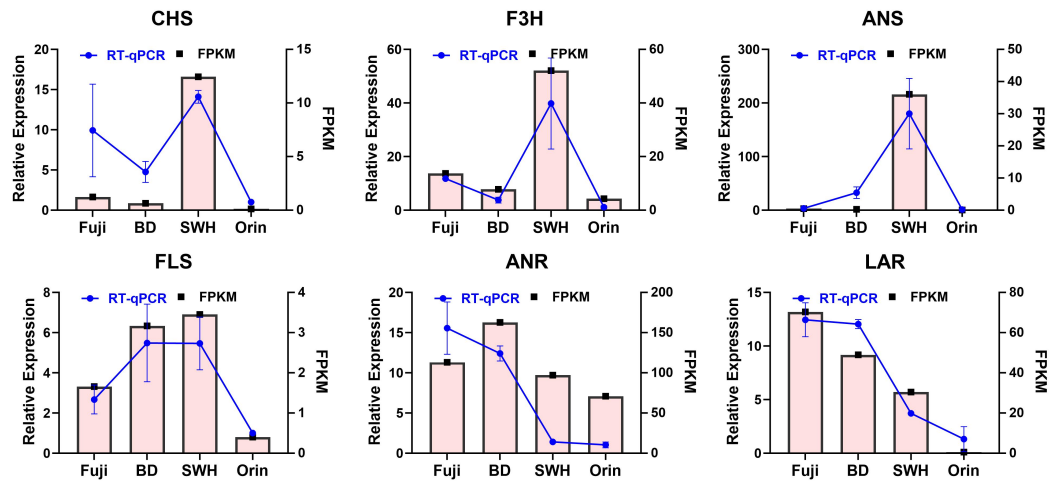
1 2 Supplementary Figure S1. RT-qPCR validation of RNA-seq data by six DEGs.
