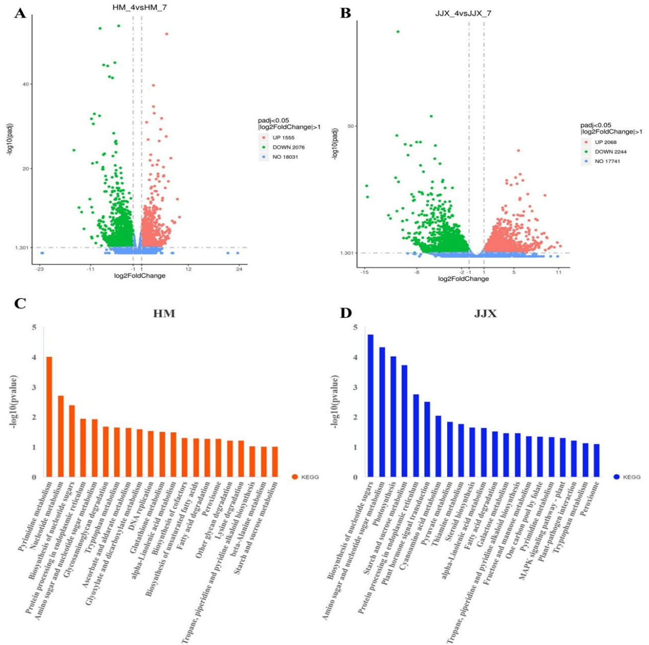
Figure S1. KEGG enrichment analysis of differentially expressed genes in wampee fruits at 78 DAB and 99 DAB. A, Volcano plot of differentially expressed genes in 'Huami' wampee. B, Volcano plot of differentially expressed genes in 'Jinjixin' wampee. C, KEGG enrichment analysis of differentially expressed genes in 'Huami' wampee. D, KEGG enrichment analysis of differentially expressed genes in 'Jinjixin' wampee. HM_4 and HM_7 represent the 78 and 99 DAB 'Huami' wampee fruits, respectively; JJX_4, JJX_7 represent the 78 and 99 DAB 'Jinjixin' wampee fruits, respectively.
