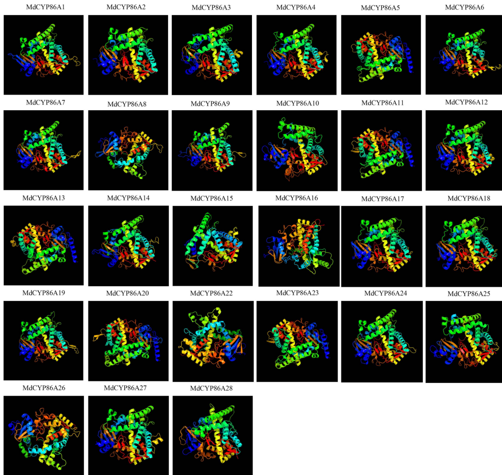
Figure S2: 3D protein structure of MdCYP86As.
