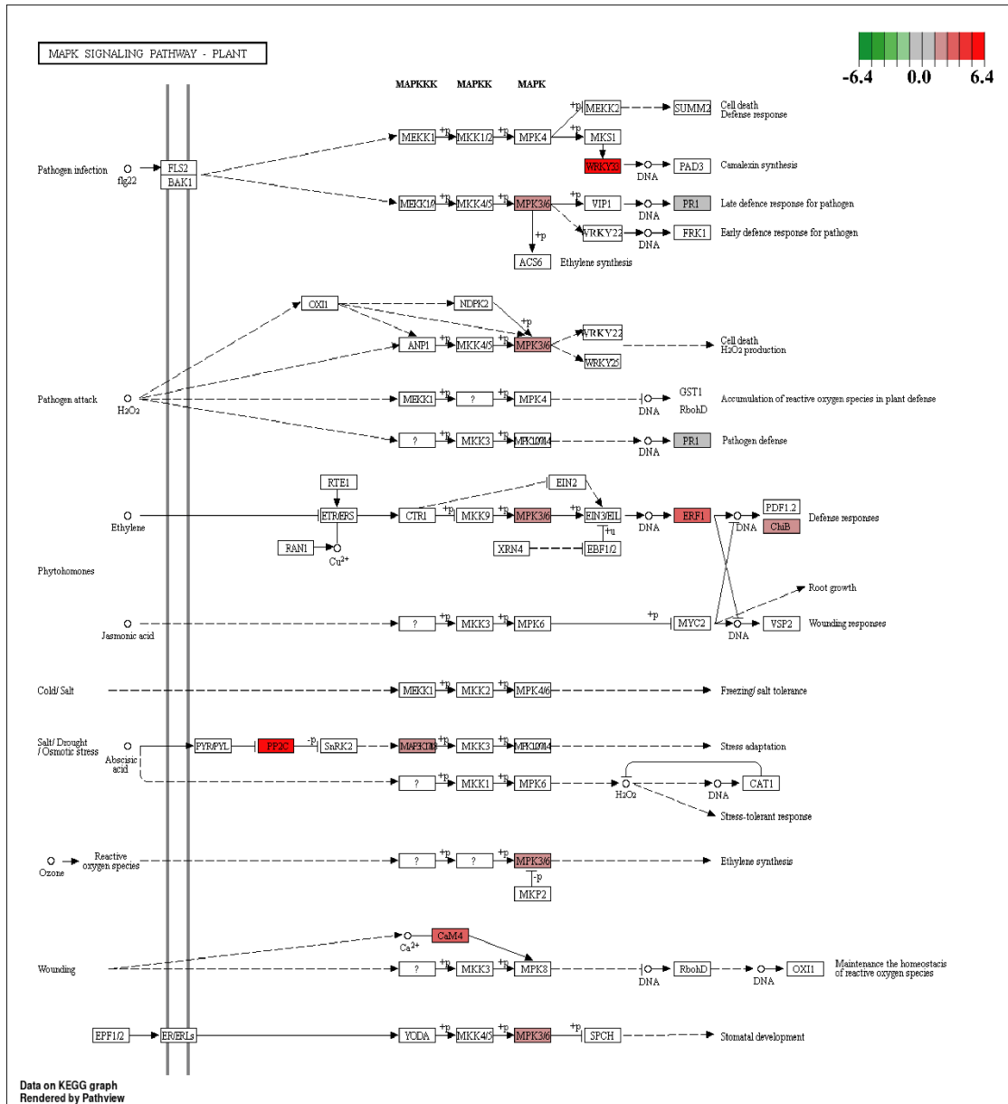
Figure S1 MAPK signaling pathway diagram. The scale in the upper right corner of the picture is the absolute value of the maximum log 2 (foldchange) annotated to this pathway for all differential genes. The red color indicates that the genes annotated to the pathway are up-regulated differential genes, and the green color indicates that the genes annotated to the pathway are down-regulated differential genes. The grey color indicates that the genes annotated to the pathway have both up-regulated differential genes and down-regulated differential genes. The white color indicates that there is no difference in the genes annotated to the pathway.
