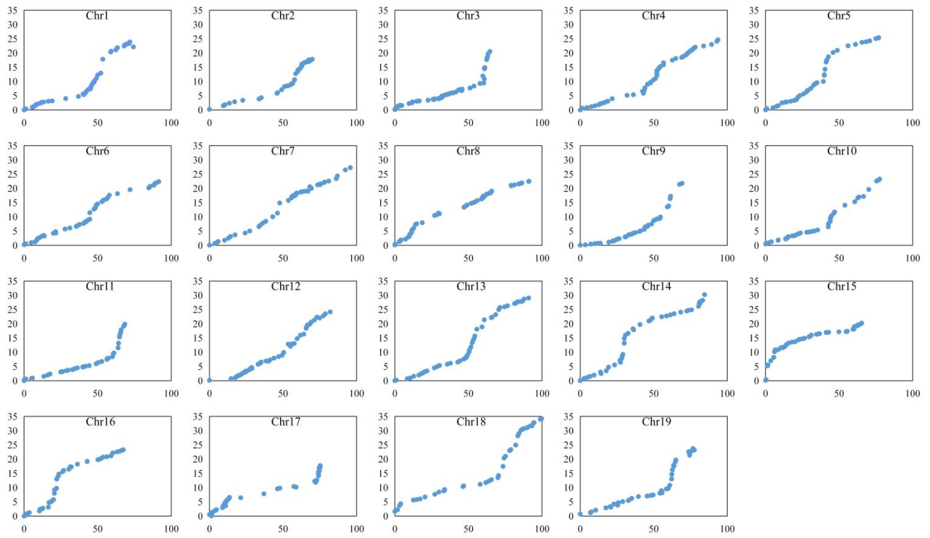
Figure S2 Collinearity analysis of the genetic map. The X axis indicates the genetic position of each SNP (cM), the Y axis indicates the physical position of each SNP (Mbp).
