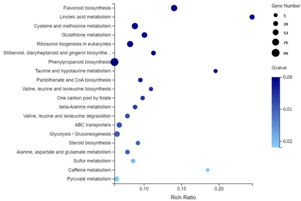
Supplementary Fig. S1 Differential gene KEGG Pathway enrichment
