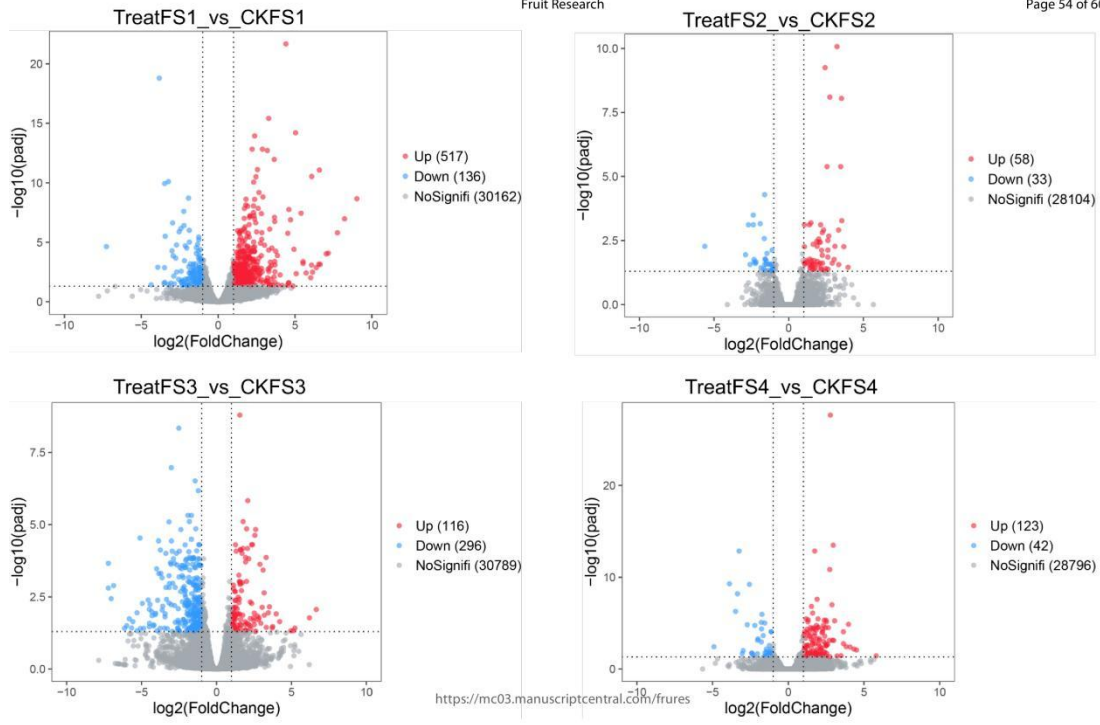
Figure S3. Volcano plot of 4 time point difference analysis
