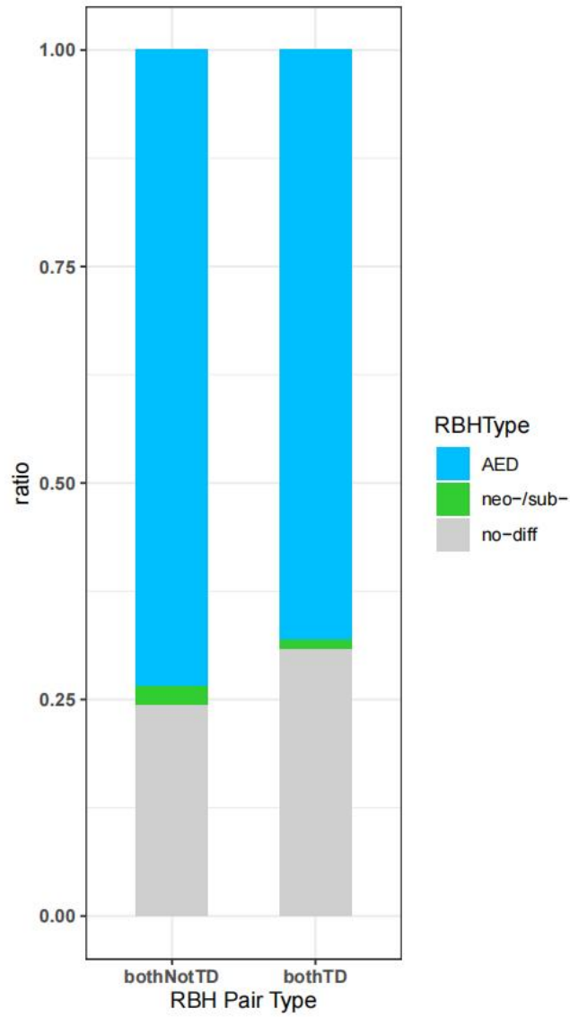
Figure S25. Classification of RBH gene pairs by expression patterns.
