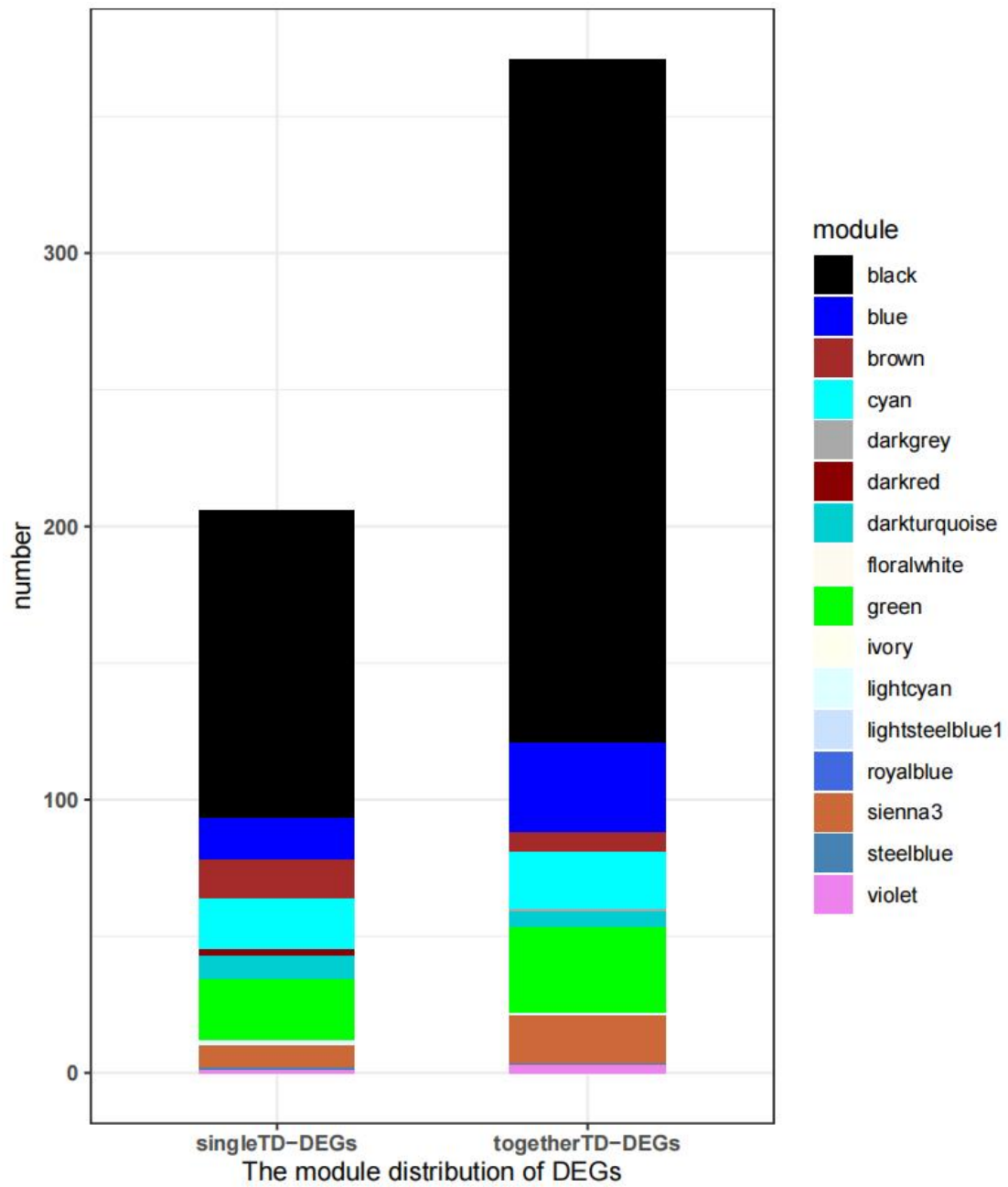
Figure S19. Modules distribution of singleTD-DEGs and togetherTD-DEGs of WGCNA analysis. By quantity.
