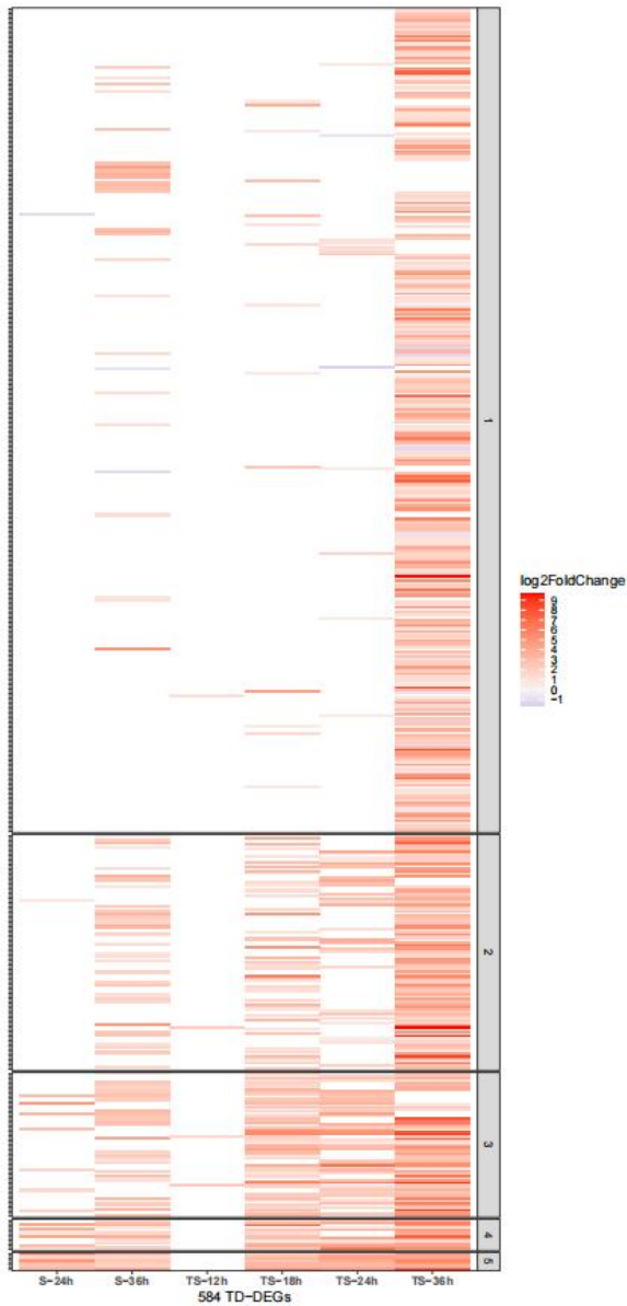
Figure S8. The heat map of log 2 foldchange (DM vs. Mock) of notTD-DEGs and TD-DEGs in different treatments.
