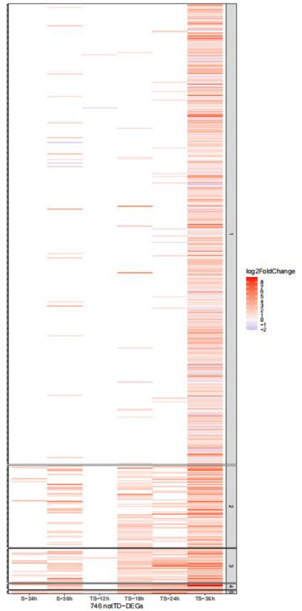
Figure S8. The heat map of log 2 foldchange (DM vs. Mock) of notTD-DEGs and TD-DEGs in different treatments.
