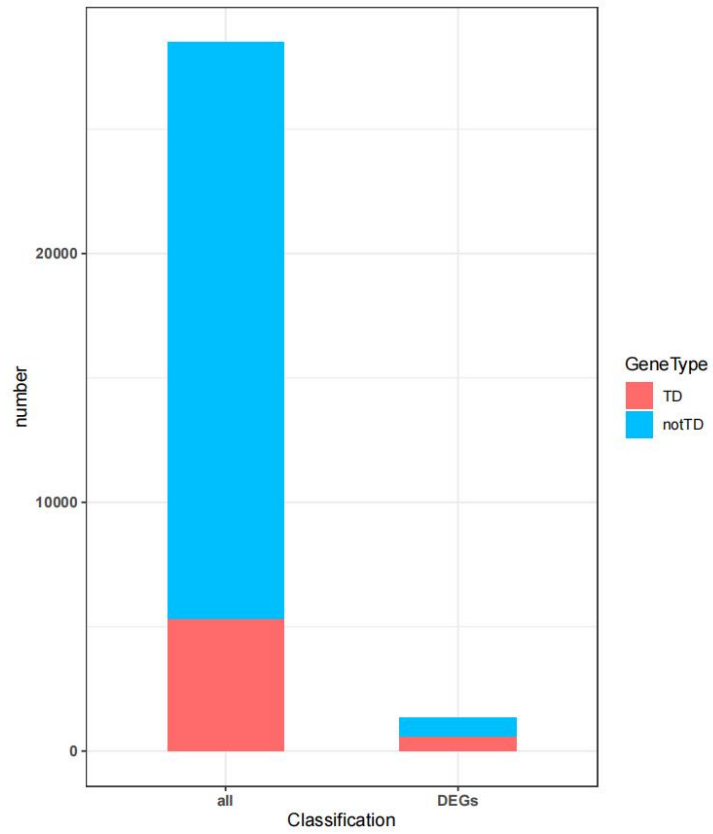
Figure S6. Distribution of TD genes and notTD genes among all genes and DEGs, respectively. By quantity.
