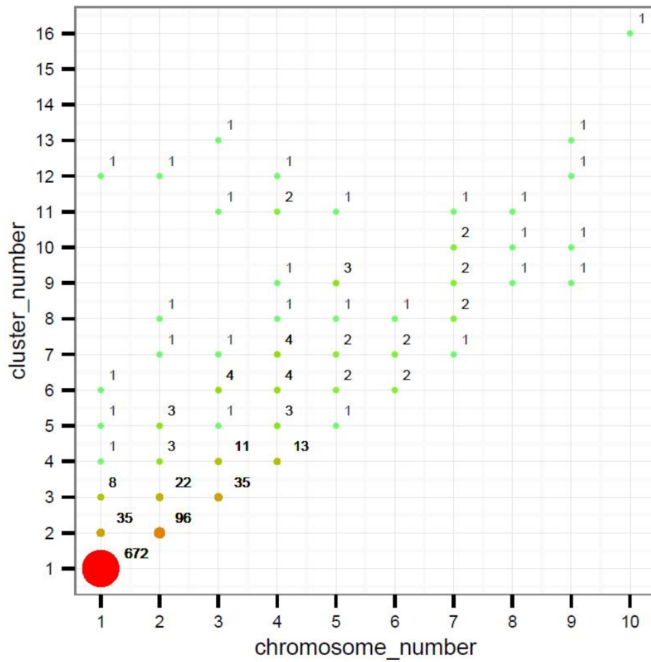
Figure S1. Number of gene clusters and chromosomal distribution of TD genes from different families.
