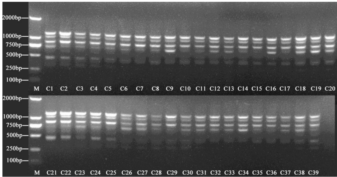
Figure S3. Electrophoresis results of 39 late-mature peach germplasm resources amplified via SRAP primer me5/em3.
