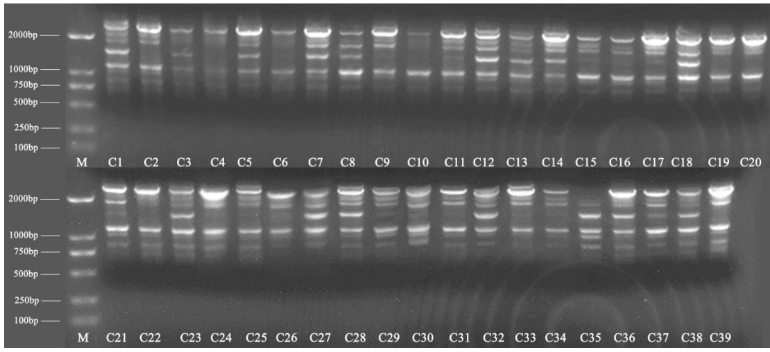
Figure S2. Electrophoresis results of 39 late-mature peach germplasm resources amplified via ISSR primer UBC855.
