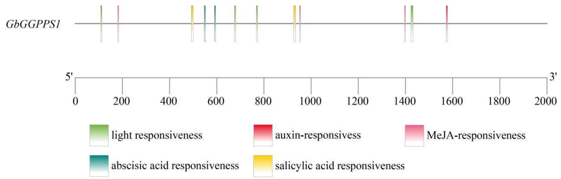
Fig. S2: Putative cis-acting regulatory elements in the GbGGPPSI promoter.
