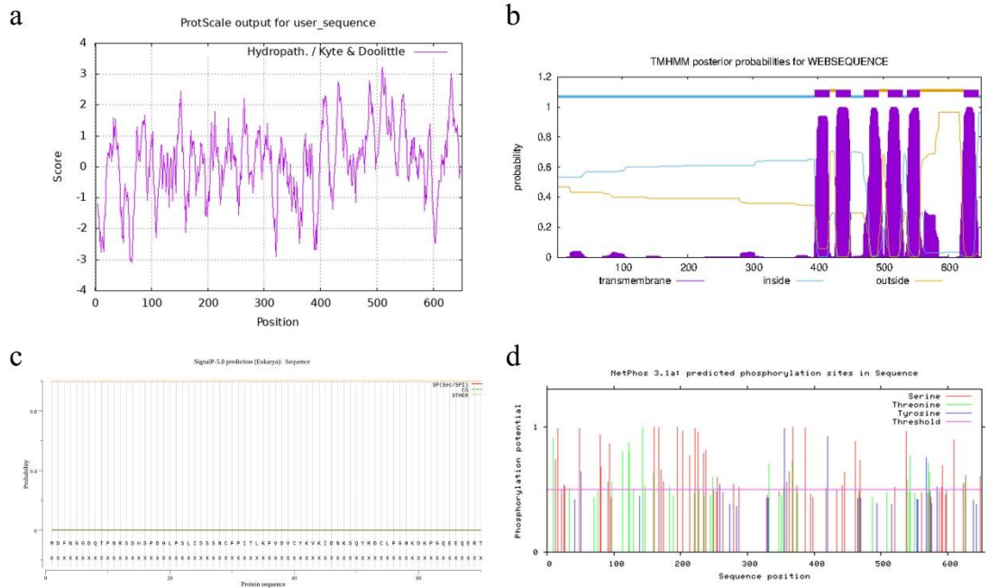
Supplementary Figure S1. Characteristics of MdABCG25 protein. (a) The hydrophaticity of MdABCG25 protein. (b) The transmembrane domains of MdABCG25 protein. (c) The signal peptides of MdABCG25 protein. (d) The predicted phosphorylation sites of MdABCG25 protein.
