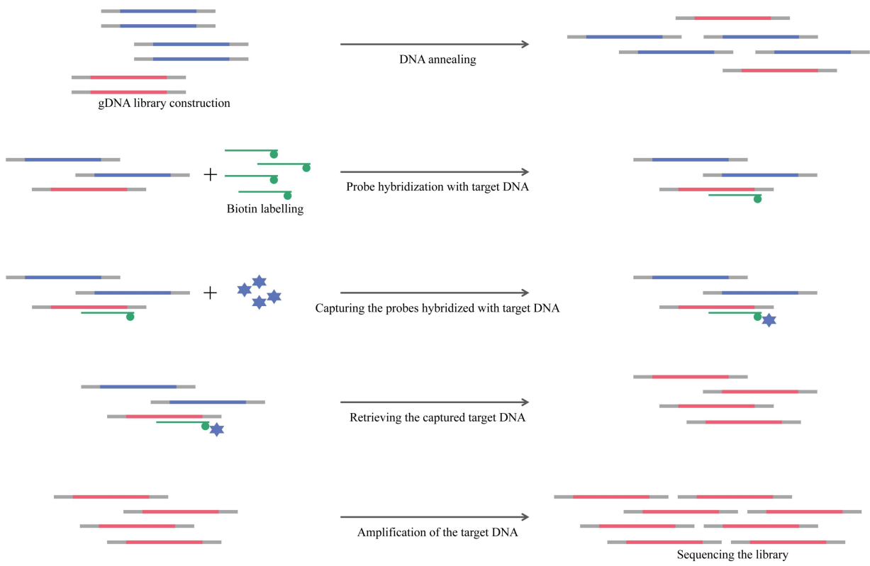
Figure S1. Flowchart for genotyping by target sequencing with GenoBaits.
