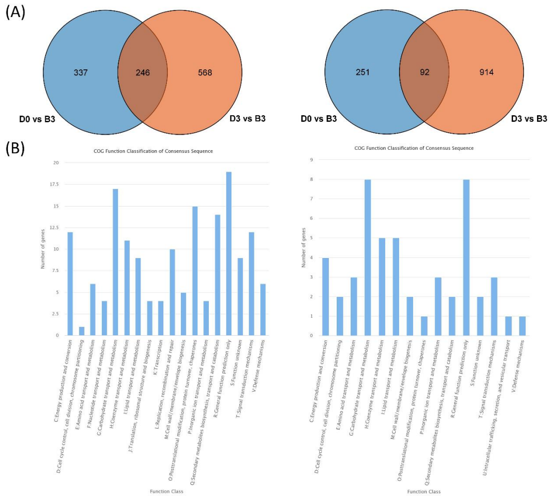
Fig. S2. Analysis of DEGs between fruit samples treated with 72h of blue light irradiation (B3) and those at 0 (D0) and 72h (D3) of treatment in dark. (A). The number of differentially up-regulated and down-regulated genes. (B) Histogram of COG function for the up-regulated and down-regulated genes.
