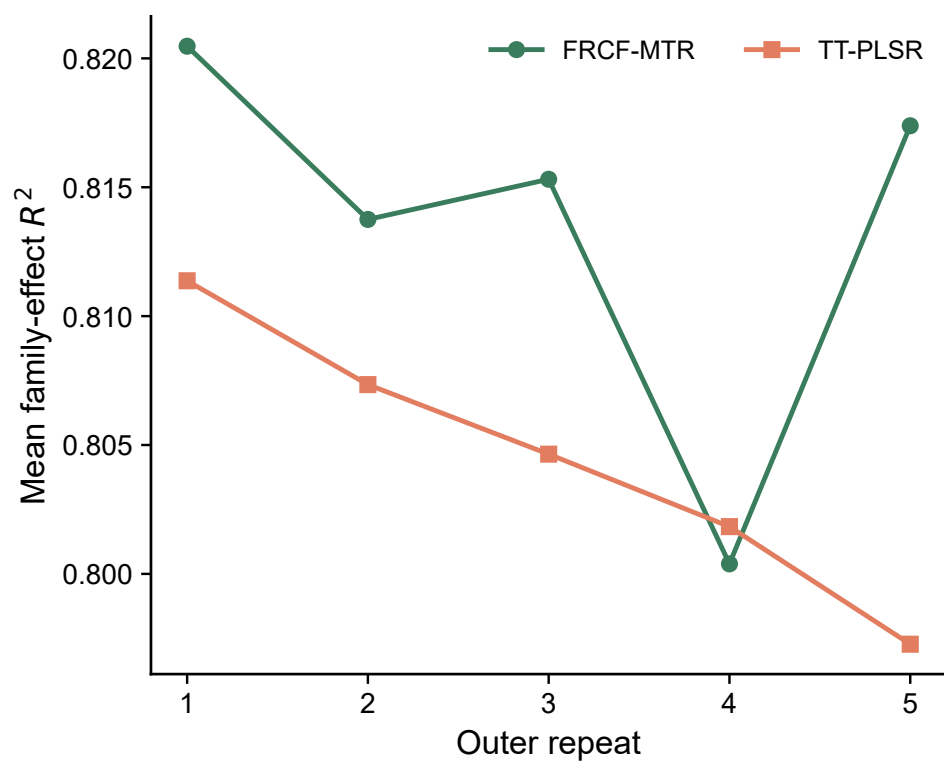
Figure S3. Repeat-wise mean family-effect R^2 and Spearman rank correlation for FRCF-MTR and TT-PLSR (PDF).
