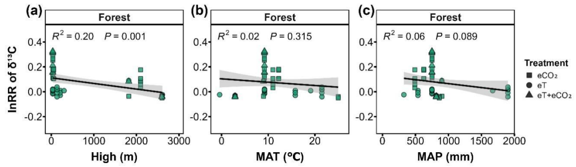
Figure S6. Relationship between the lnRR of \delta^{13}\text{C} (carbon stable isotope composition) and (a) high, (b) mean annual temperature (MAT), and (c) annual average precipitation (MAP).
