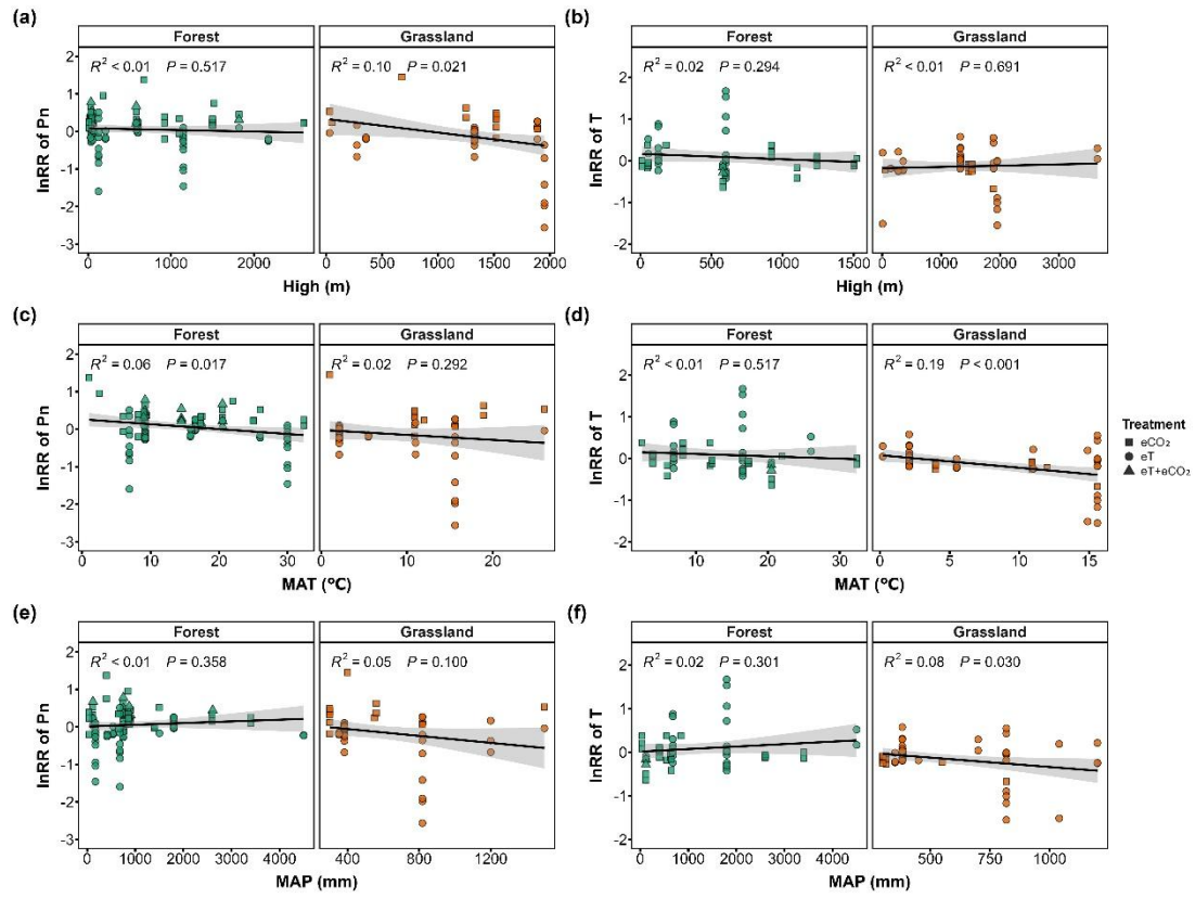
Figure S5. Relationship between the lnRR of Pn, T and (a, b) high, (c, d) mean annual temperature (MAT), and (e, f) annual average precipitation (MAP).
