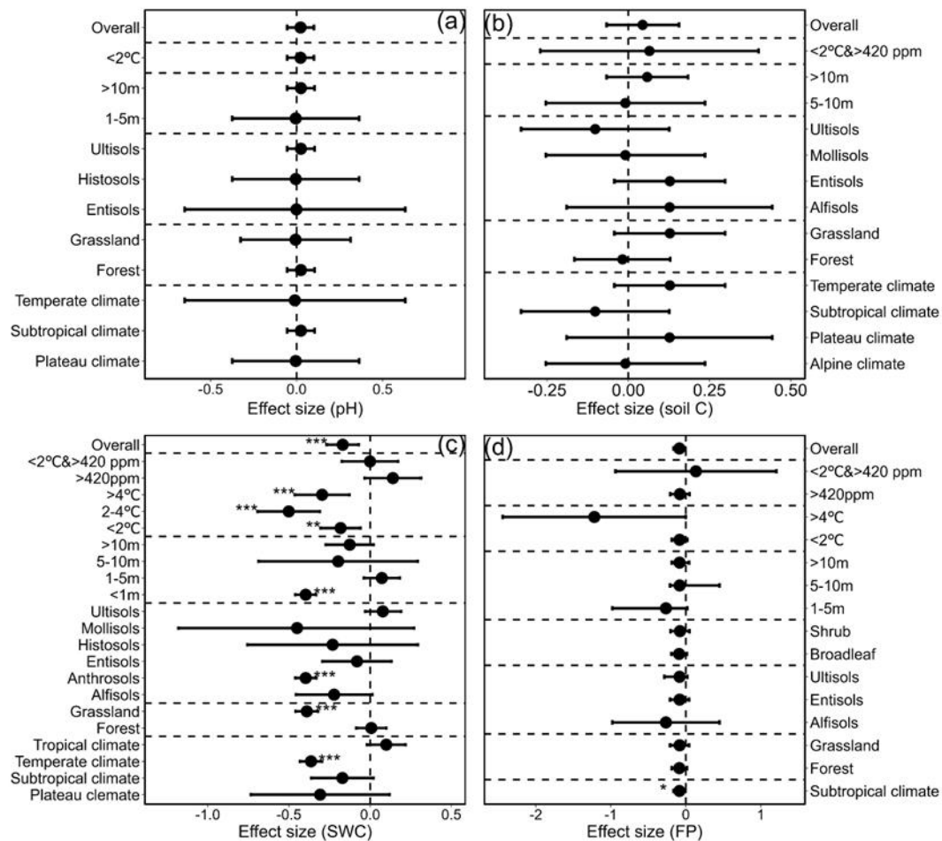
Figure S4. Subgroup effect size of warming treatment (intensity and duration), ecosystems, soil texture and plant types on soil properties (a, pH; b, soil C; c, SWC) and leaf P content (d) in forest and grassland. Values represent lnRR and 95% CIs. * indicates a significant correlation at P < 0.05 level, ** indicates an extremely significant correlation at P < 0.01 level, and *** indicates an extremely significant correlation at P < 0.001 level.
