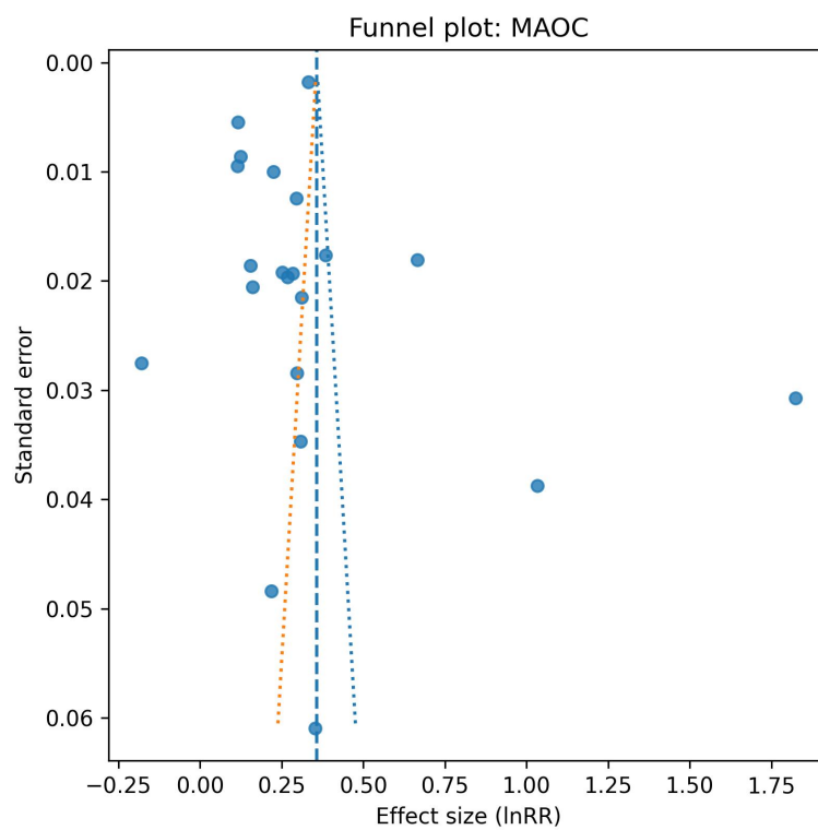
Figure S4. Funnel plot for MAOC.
