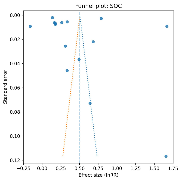
Figure S2. Funnel plot for SOC.
