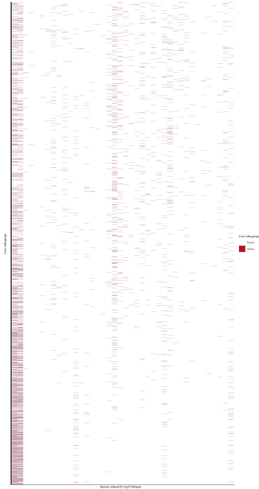
Figure S3. Species-level presence and absence of core orthogroups. Heatmap showing the distribution of core orthogroups across the 40 species. Species are ordered from low to high log10-transformed lifespan along the horizontal axis. Rows represent core orthogroups that are absent from at least one species. White cells indicate that the orthogroup is present, whereas red cells indicate that it is absent.
