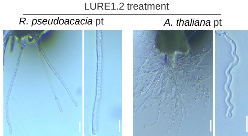
Fig. S5 R. pseudoacacia pollen tubes do not respond to AtLURE1.2.
