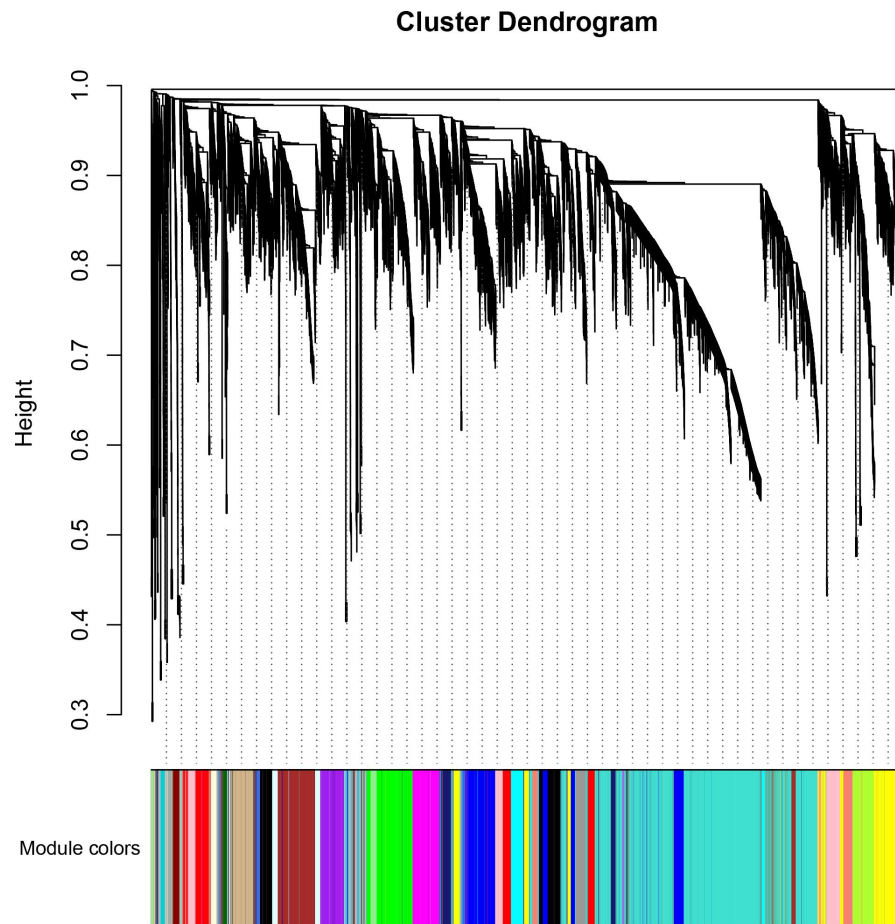
Figure S3 WGCNA cluster dendrogram and module assignment. Top: Cluster dendrogram (vertical "Height" = dissimilarity between gene clusters). Bottom: Color-coded co-expression modules (each color = a gene group with similar expression patterns).
