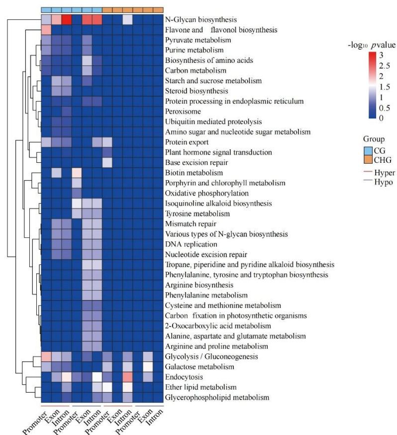
Fig. S5 KEGG functional enrichment analysis of hyper- and hypo-promoter/exon/intron-DMDGs in the CG-blue and CHG-blue clusters.
