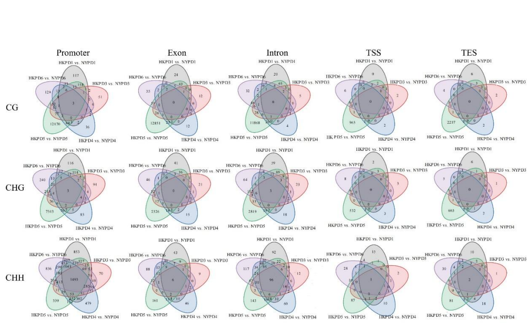
Fig. S3 Venn diagrams of DMGs across different sequence contexts and functional regions in five comparison groups.
