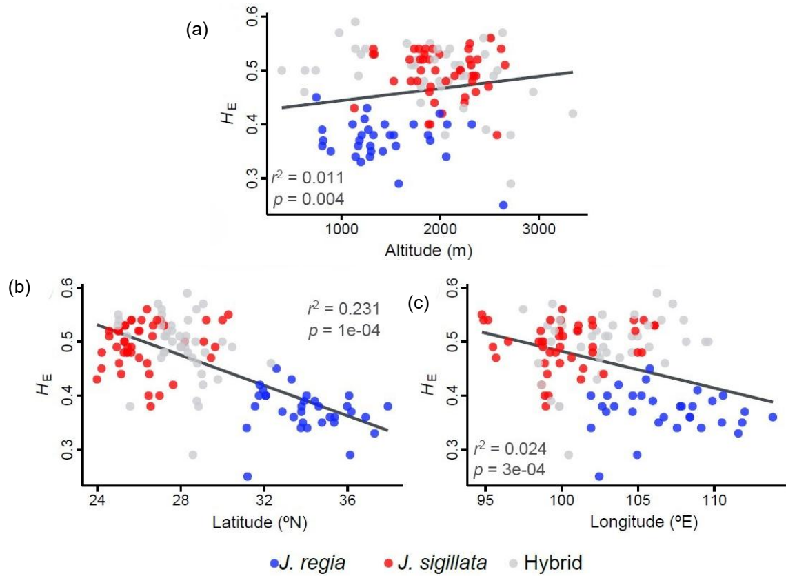
Fig. S2 Genetic differentiation and diversity in relation to geography. (a) Correlation between genetic diversity ( H_E ) and altitude; (b) Correlation between genetic diversity ( H_E ) and latitude; (c) Correlation between genetic diversity ( H_E ) and longitude.
