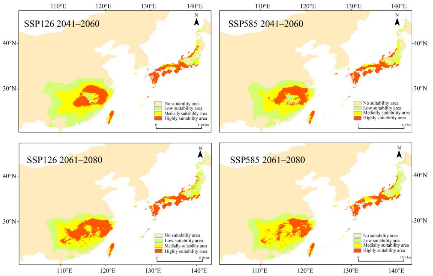
Supplementary Fig. S9 Simulation of ecological niches of Q. gilva using Maxent across four time periods: SSP126 2041–2060, SSP585 2041–2060, SSP126 2061–2080, and SSP585 2061–2080.
