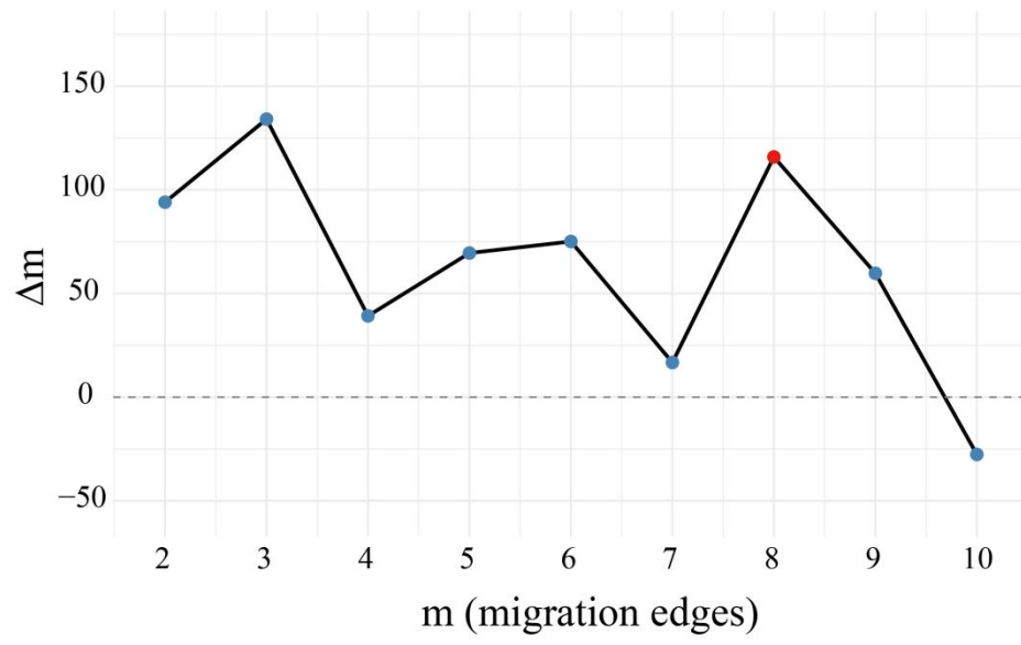
Supplementary Fig. S5 Distribution of \Delta m inferred by OptM.
